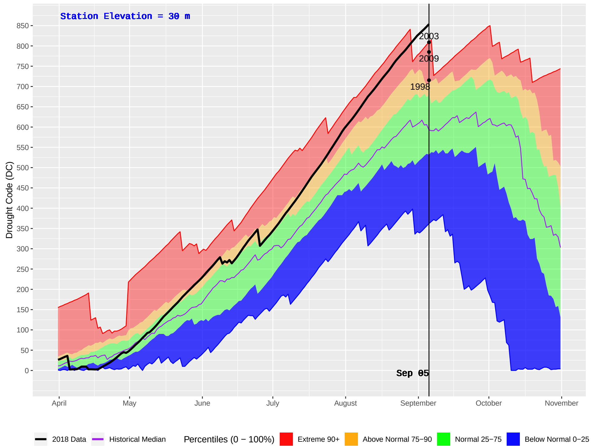
CEDAR (59) : Historical (1989–2016) and Current (2018) Daily Drought Code (DC)
